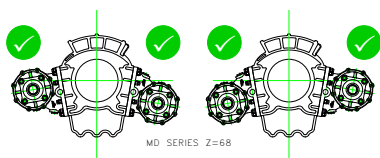
PTO MOUNTING POS. 1
