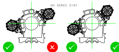
PTO MOUNTING POS. 1
